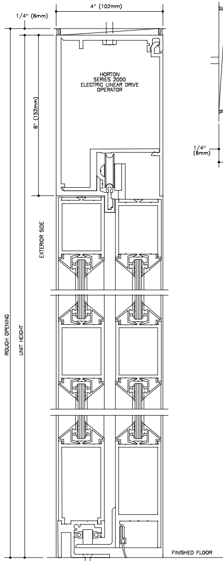
VERTICAL SECTION FULL SCALE
