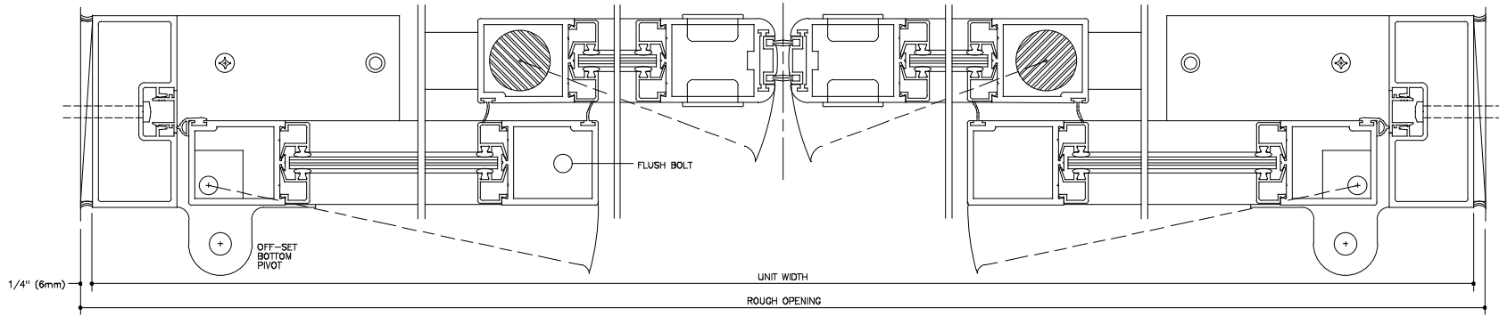
HORIZONTAL SECTION FULL SCALE
