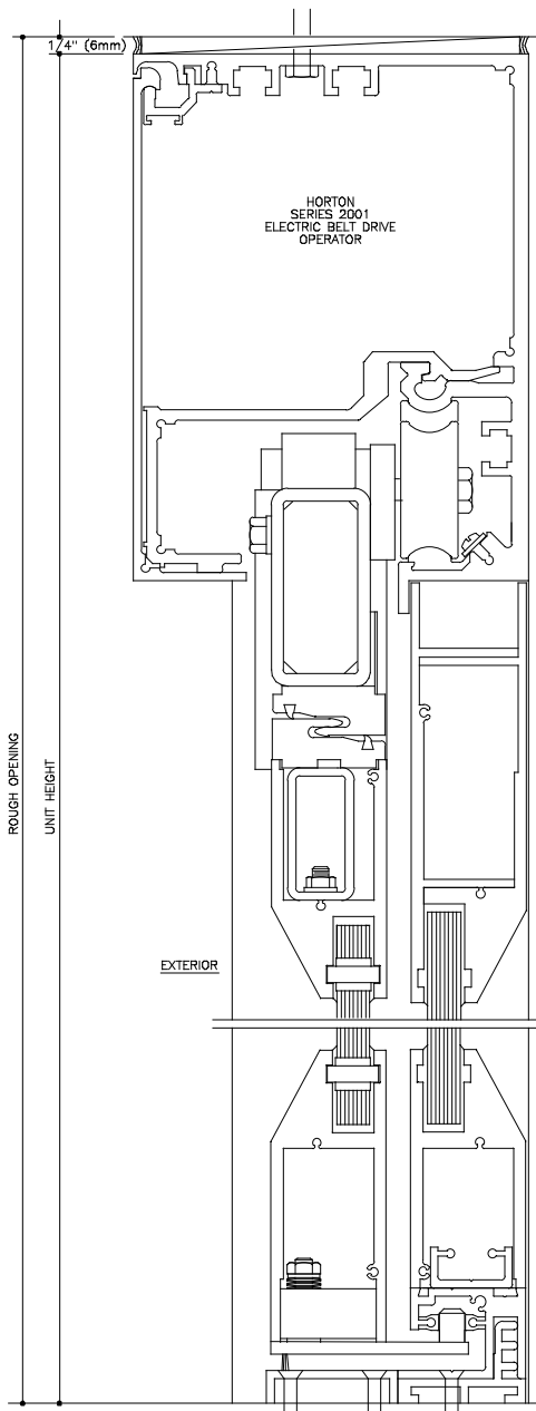
1 VERTICAL SECTION FULL SCALE DOOR SHOWN IN OPEN POSITION
